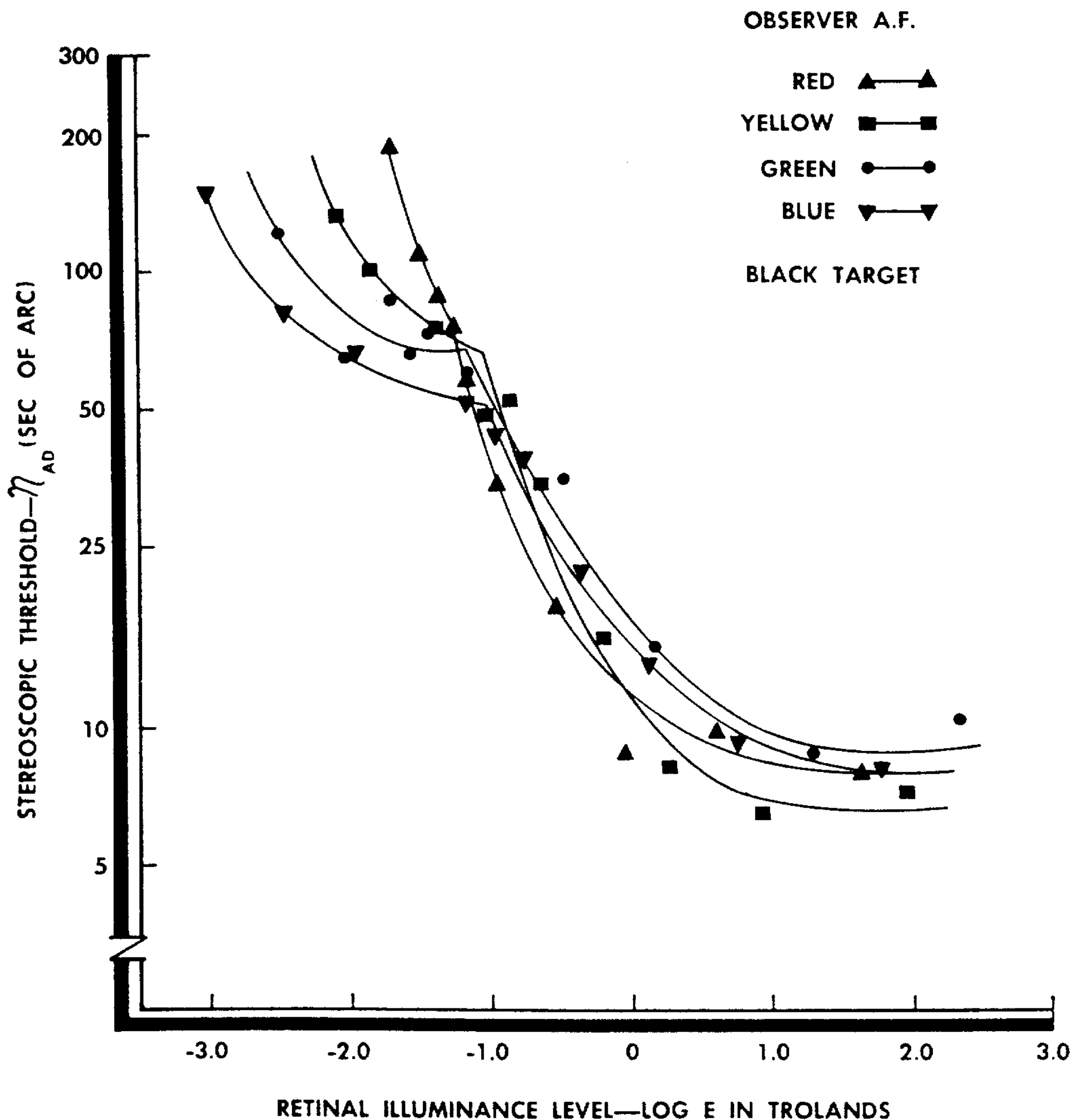
Fig. 1. Stereoscopic threshold angle, \eta_{AD} , in logarithmic scale, as a function of retinal illuminance, \log E , in trolands. Each data point for observer A.F. is based on the mean value of the average deviation of four groups of 14 equidistance settings.
