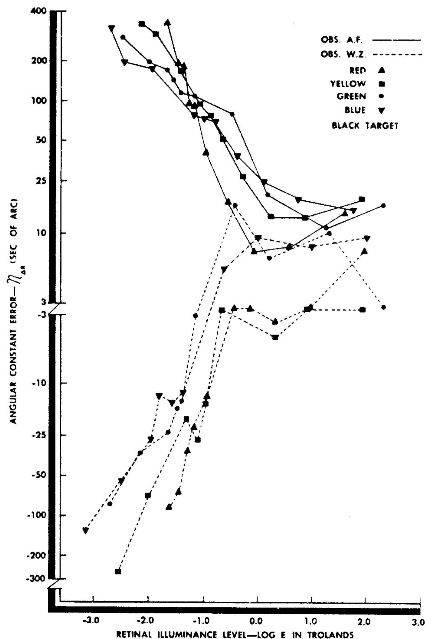
Fig. 3. Angular constant error, \eta\Delta_R , in logarithmic scale, as a function of retinal illuminance, \log E , in trolands. Each data point for the two observers is based on the average value of the mean of four groups of 14 equidistance settings.
