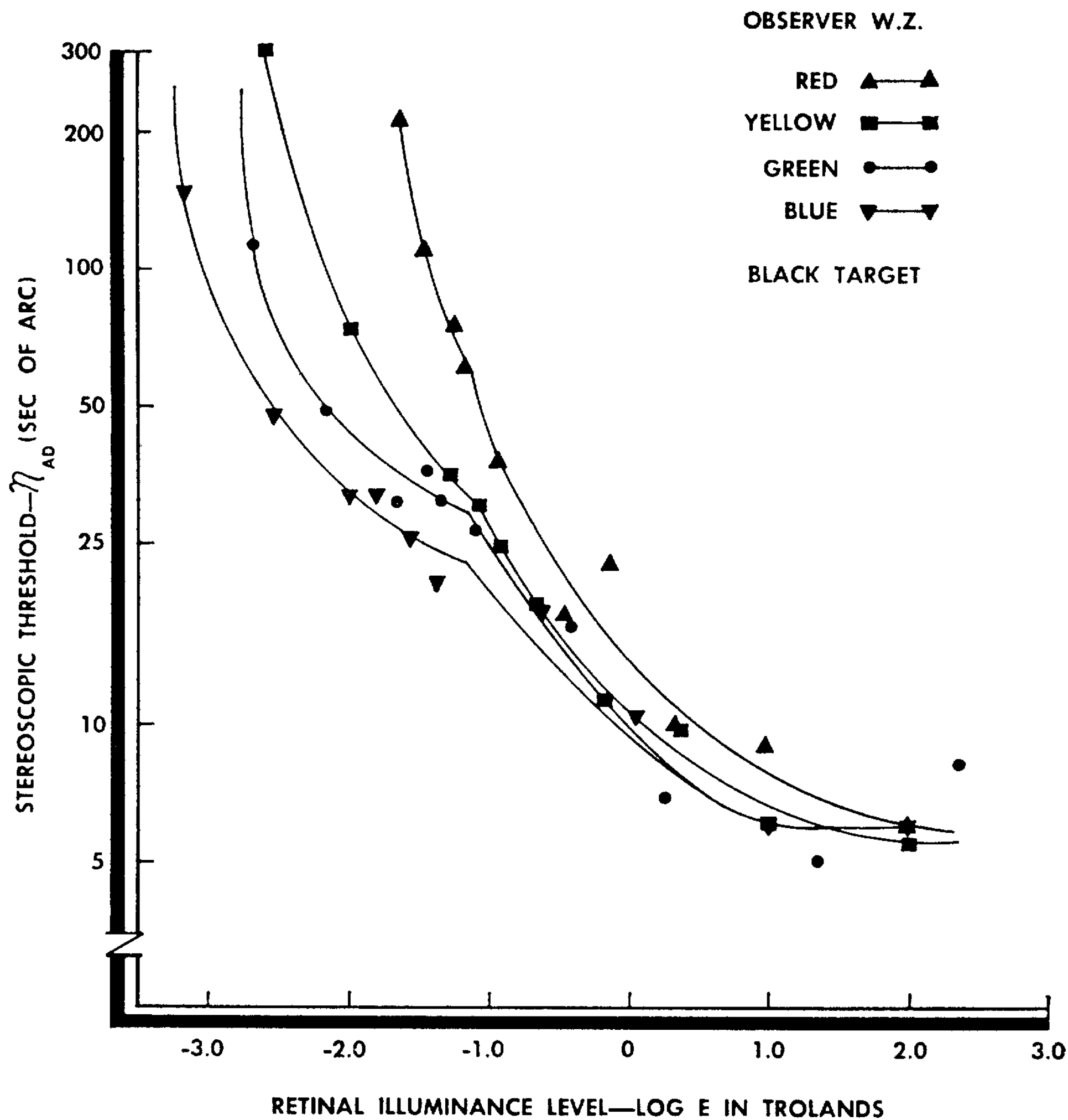
Fig. 2. Stereoscopic threshold angle, \eta_{AD} , in logarithmic scale, as a function of retinal illuminance, \log E , in trolands. Each data point for observer W.Z. is based on the mean value of the average deviation of four groups of 14 equidistance settings.
