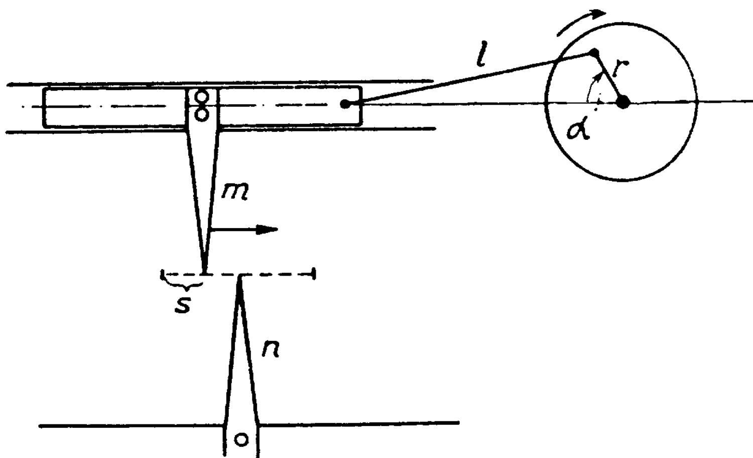
Fig. 3. Mechanism of Pulfrich's second model.
