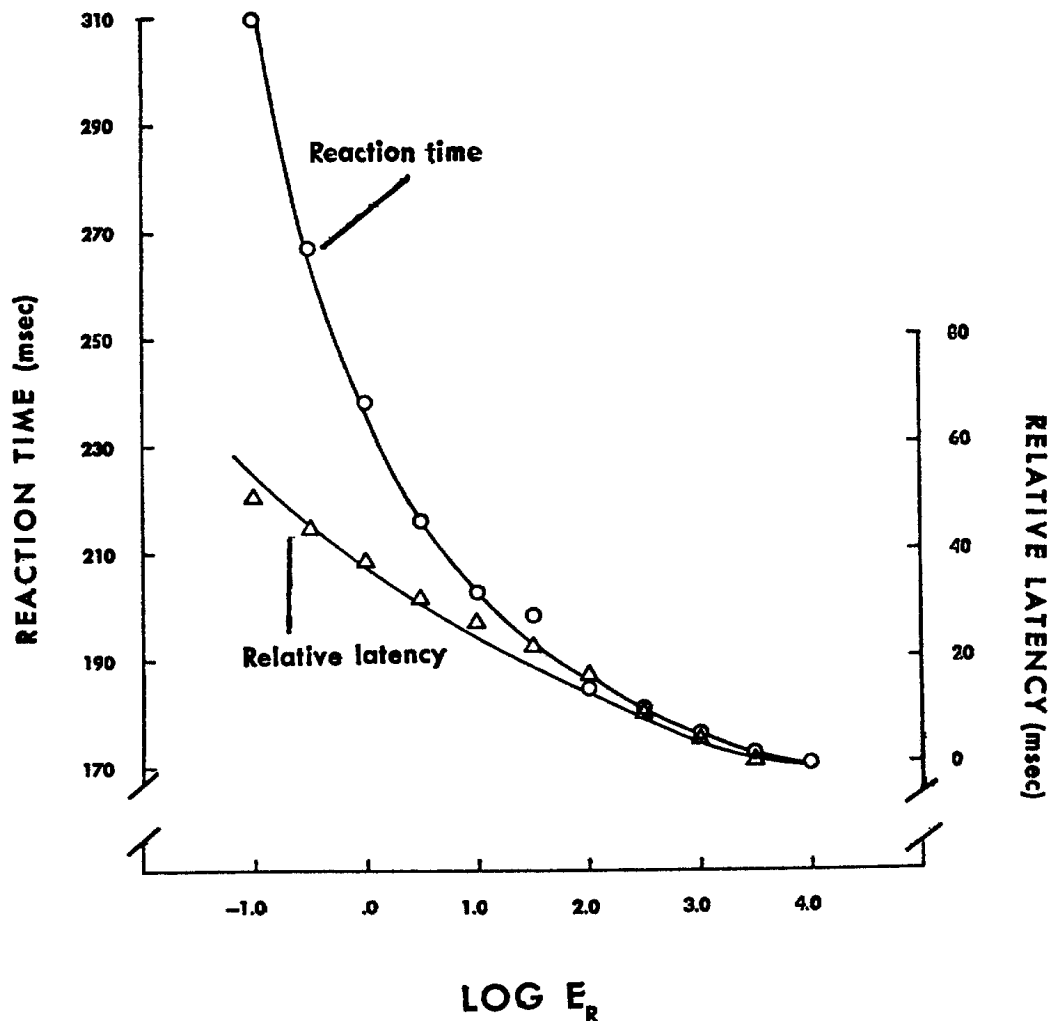
Figure 2. Average median reaction time (circles) and relative latency based on the Pulfrich settings (triangles) plotted as function of level of illumination, \log E_R . The curves represent the combined data of two observers, W.D. and A.M.
