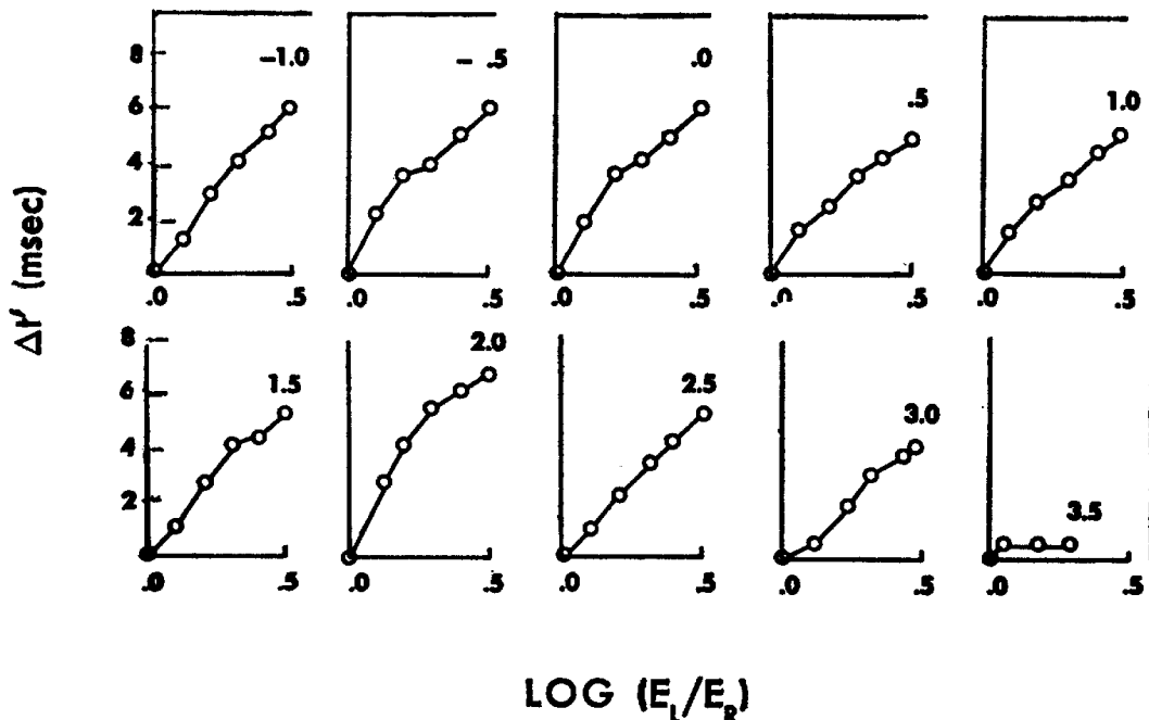
Figure 1. Average latency differences, \Delta t' , as a function of inequality of binocular illumination, \log (E_L/E_R) . The curve for each of the 10 levels of illumination, \log E_R , represents the combined data of two observers, W.D. and A.M.
